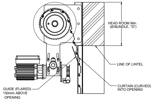
LIMITED HEAD ROOM
