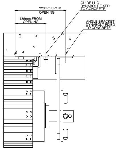
CONCRETE STRUCTURE FIXING
