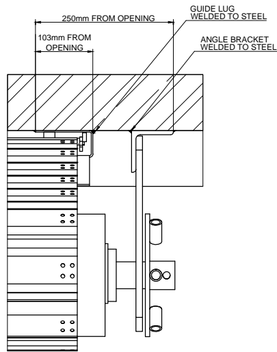
STEEL STRUCTURE FIXING
