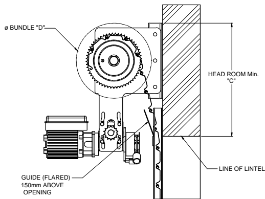
STANDARD HEAD ROOM
